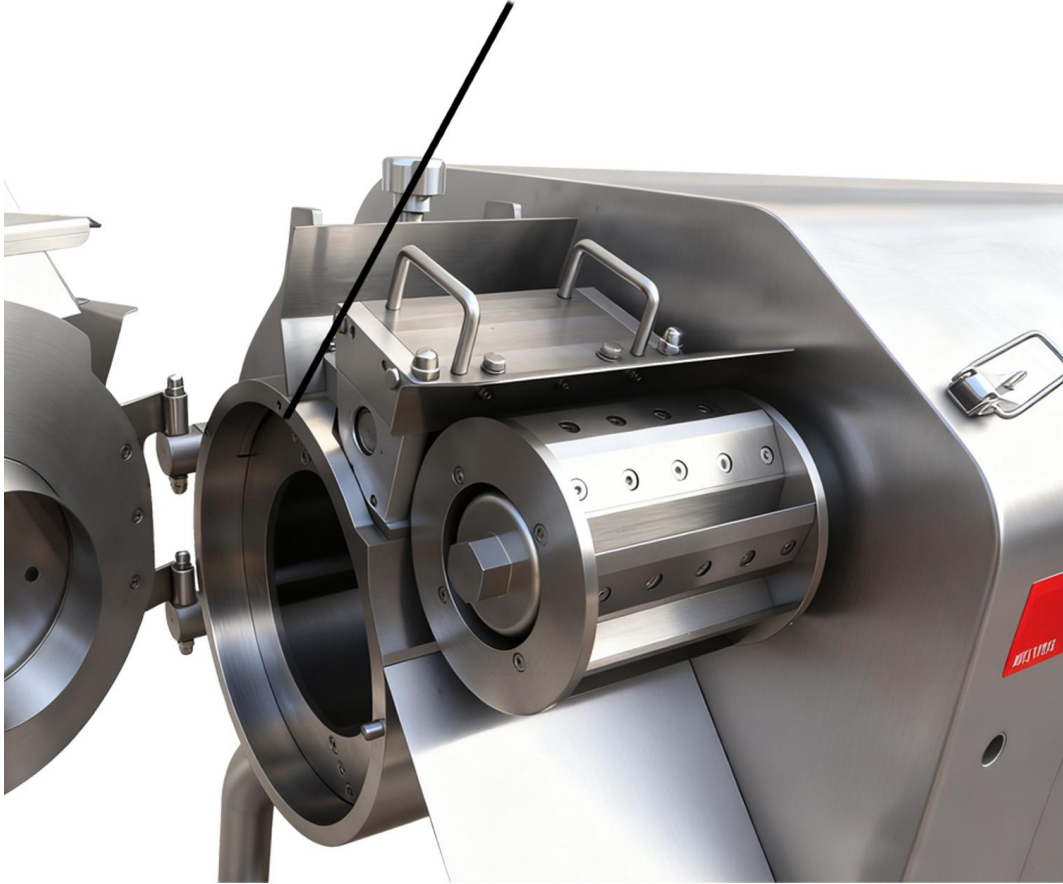
Centrifugal drum
